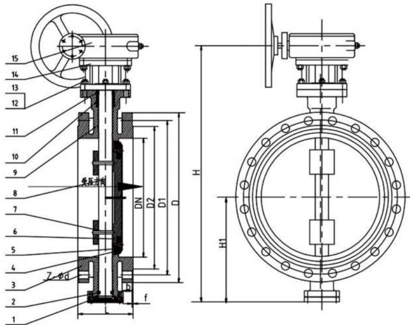
Main out-form and connection dimensions
